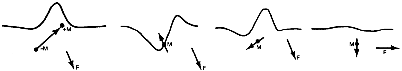
Figure 43. Total Intensity Signatures at Various Inclinations of the Field and for induced or Permanent Magnetic Moments
