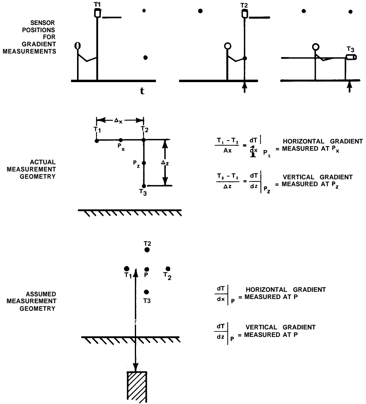
Figure 49. Gradiometer Measurement Procedures
